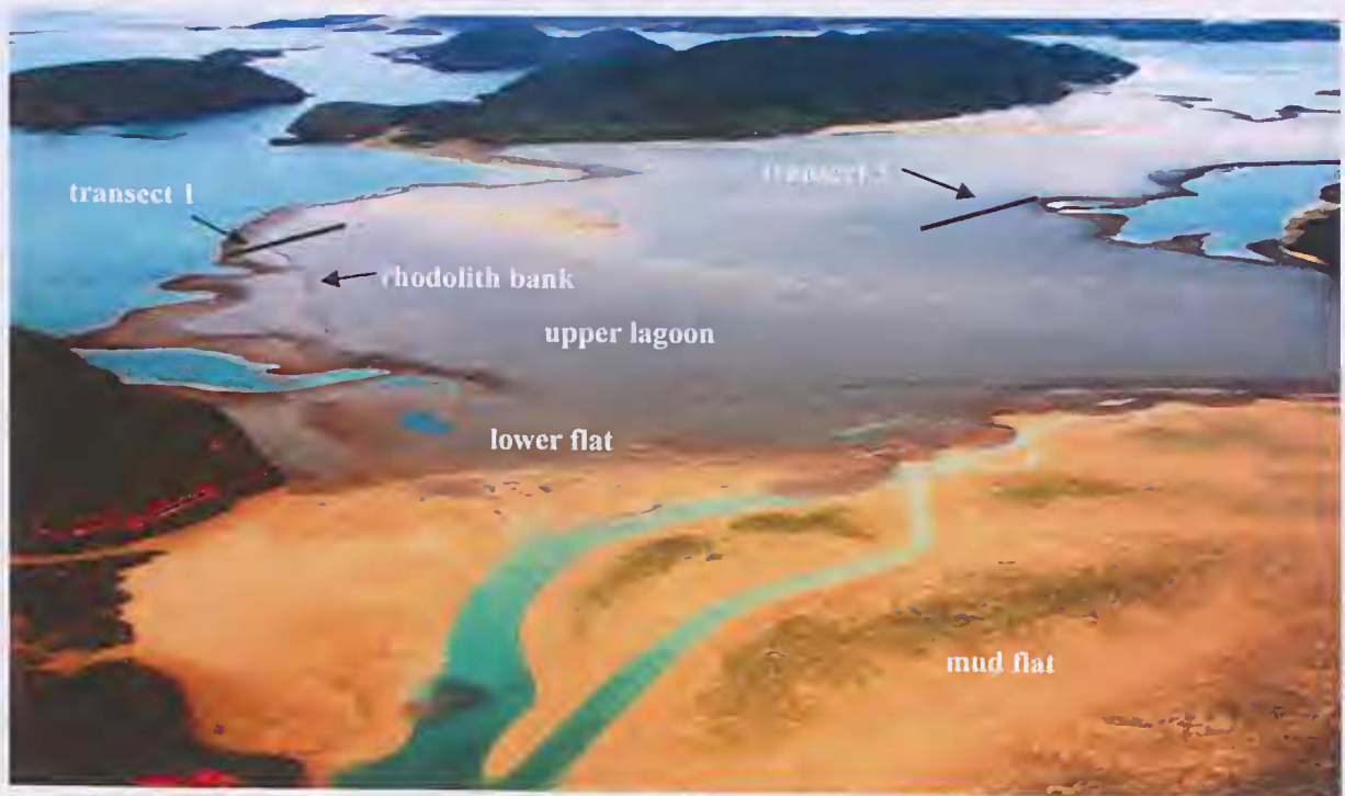
Figure 2. Low-tide aerial oblique view of South Turtle Reef, looking west. Molema Island is almost out of view on the right side. Note the massive mud bank in the foreground that overlaps the eastern margin of the reef platform [Photo: courtesy Kimberley Media and WAMSI].
